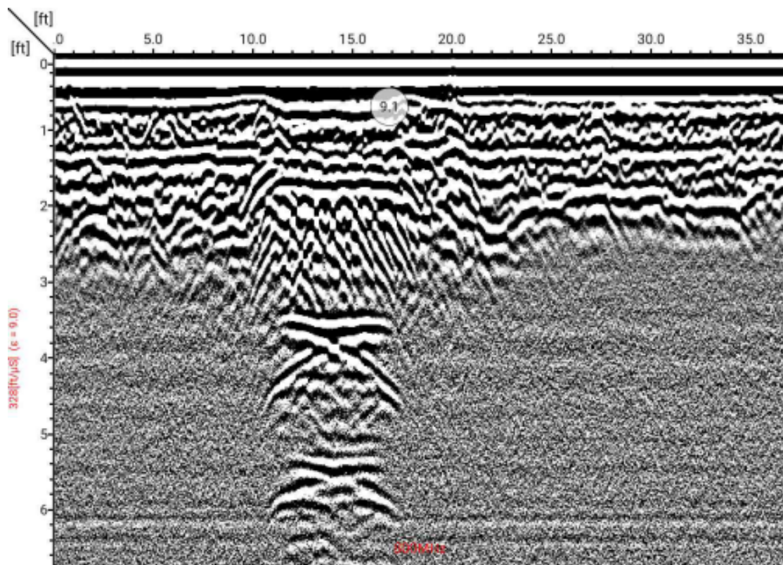
Ground Penetrating Radar (GPR) Image – East of Chase St.
