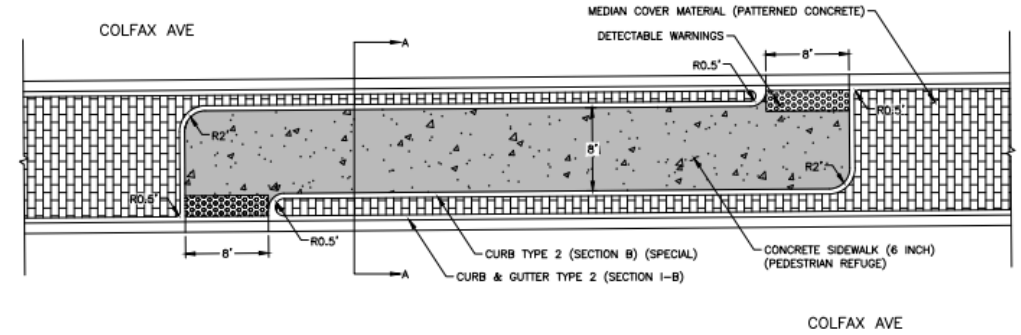
Z-CROSSING PLAN VIEW SCALE: 1" = 10'
