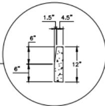
CURB TYPE 2 (SECTION B) (SPECIAL)
