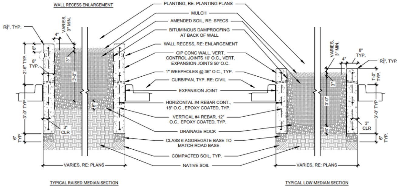
TYPICAL RAISED MEDIAN SECTION
